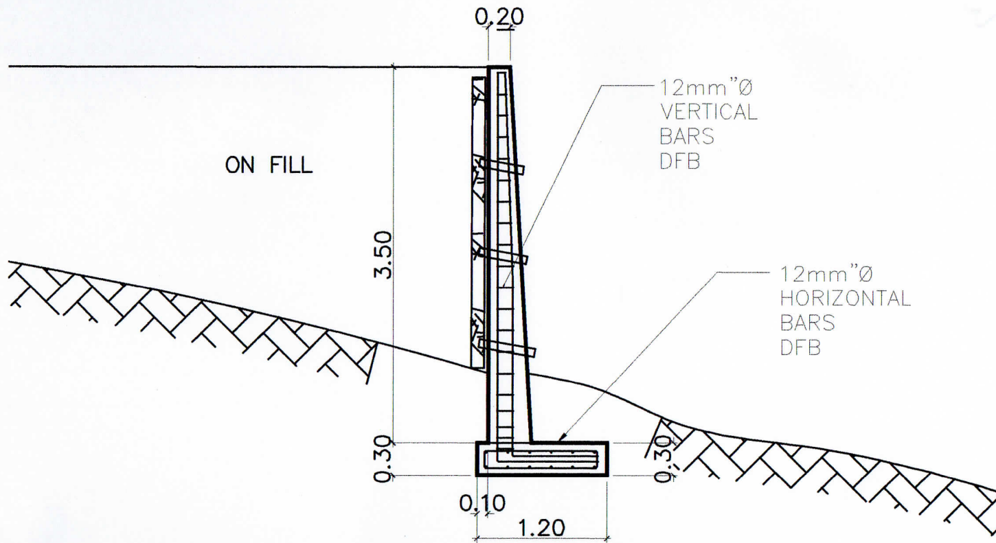
RETAINING WALL CROSS SECTION
